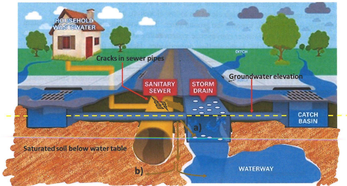
Figure III.7 Flow diagram showing possible water pathways into and out of conveyance system. a) emphasizes the possibility of leaks from the sanitary sewer contaminating groundwater and flowing into the perforated pipes of the storm conveyance system, b) emphasizes the possibility of leaks from the sanitary sewer contaminating groundwater that flows directly to the waterway.
