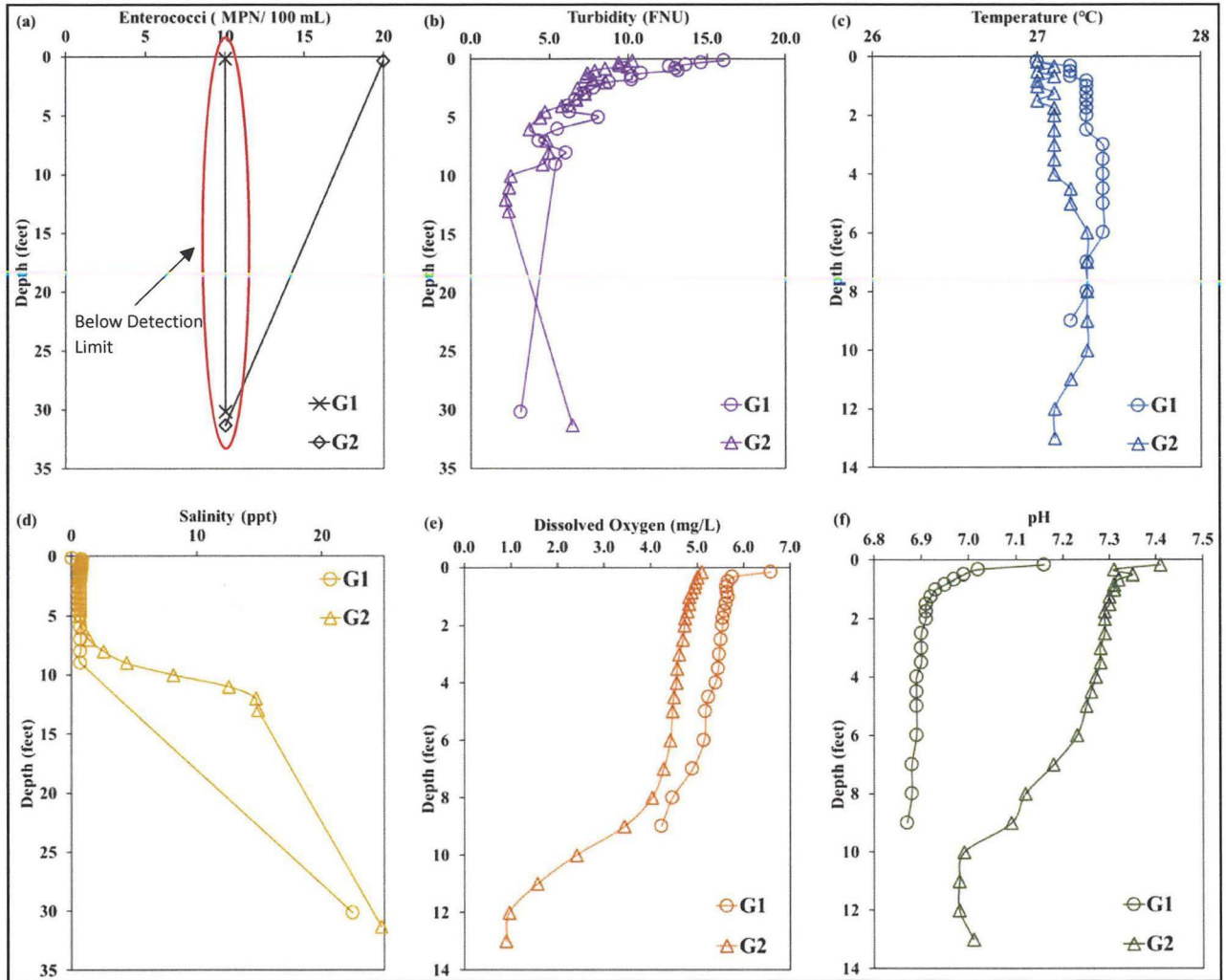
Figure V.17: Groundwater measurements at stations G1 (Bandshell) and G2 (Parkview Island) collected on November 14, 2022. Panel (a) enterococci concentration; Panel (b) turbidity; Panel (c) temperature; Panel (d) salinity; Panel (e) dissolved oxygen; and Panel (f) pH.
