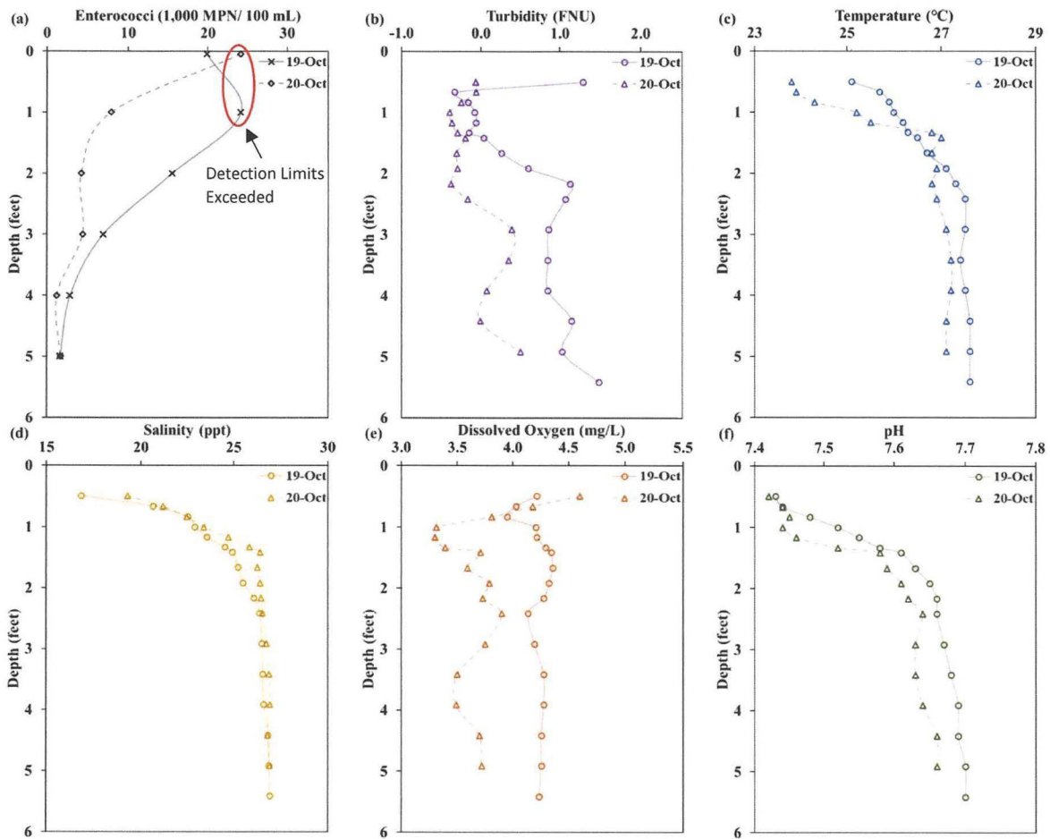
Figure V.14: Measurements versus depth at the KLRW. Panel (a) enterococci concentrations; Panel (b) turbidity; Panel (c) temperature; Panel (d) salinity; Panel (e) dissolved oxygen; and Panel (f) pH.
