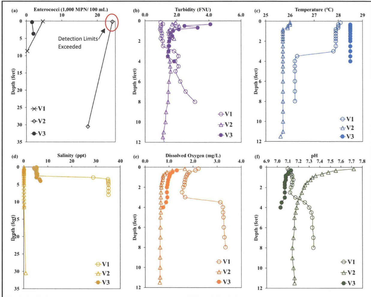
Figure V.16: Vertical drainage wells measurements (V1, V2 and V3) collected on November 14, 2022. Panel (a) enterococci concentration; Panel (b) turbidity; Panel (c) temperature; Panel (d) salinity; Panel (e) dissolved oxygen; and Panel (f) pH.
